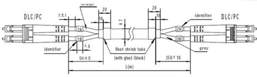
Figure Optical fiber Cable Assembly
